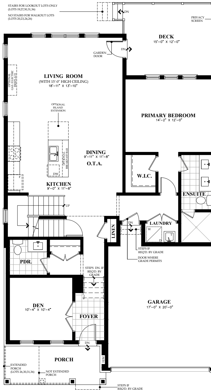
MAIN FLOOR
