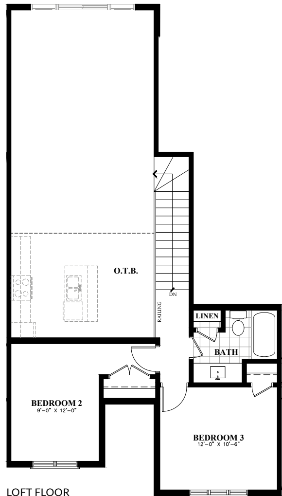
LOFT FLOOR
