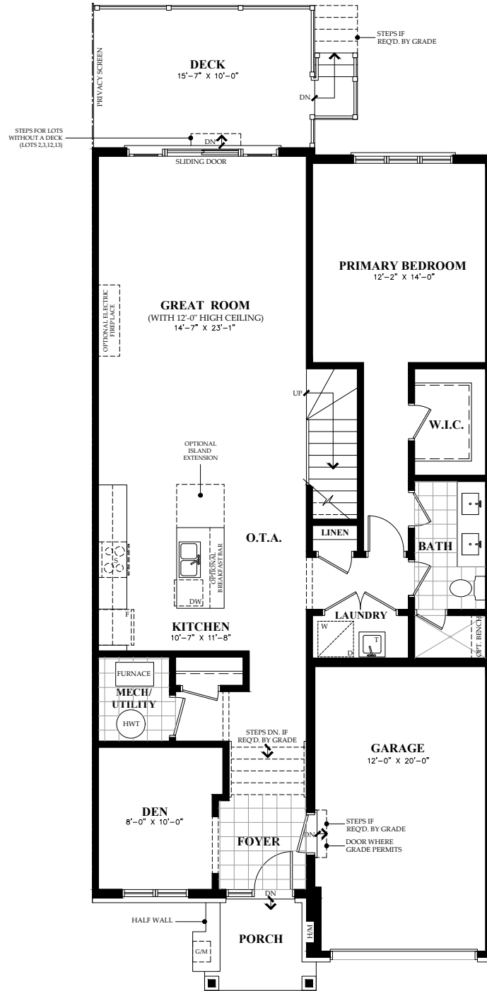
MAIN FLOOR
