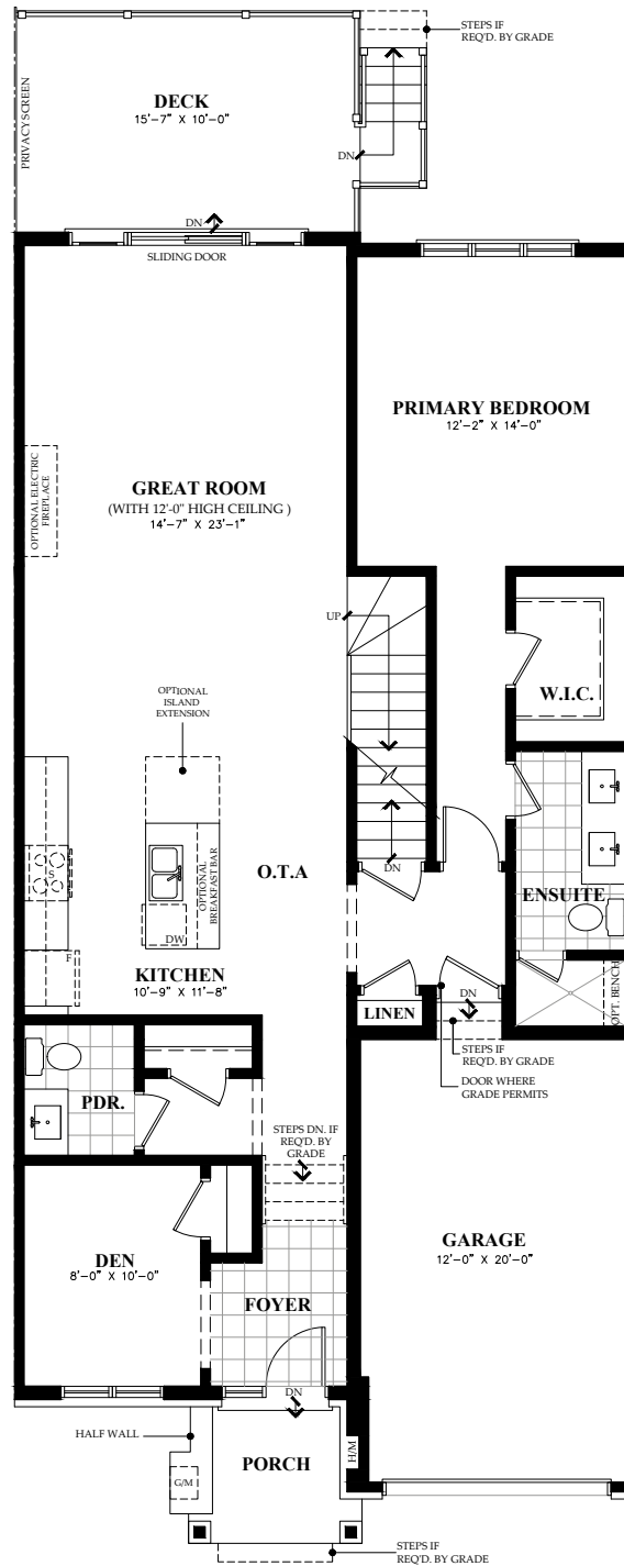
FIRST FLOOR
