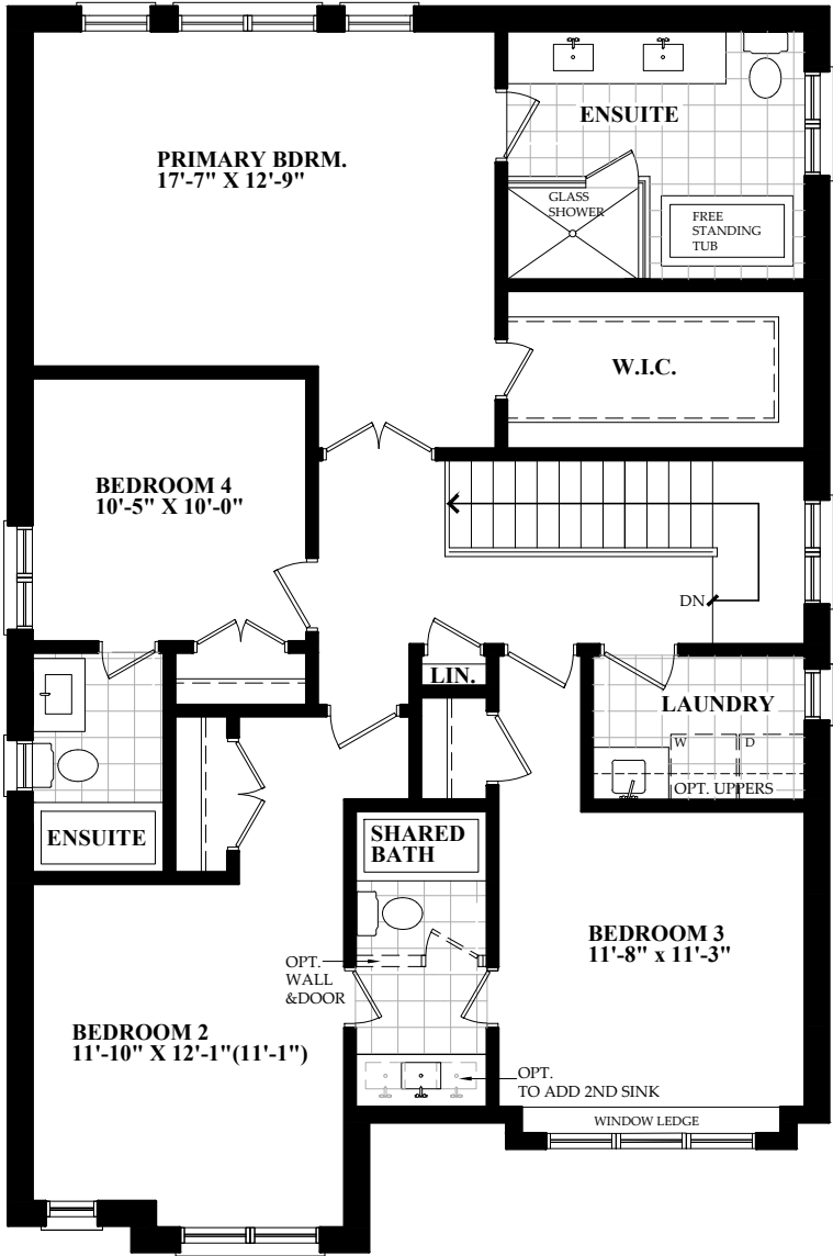
SECOND FLOOR
