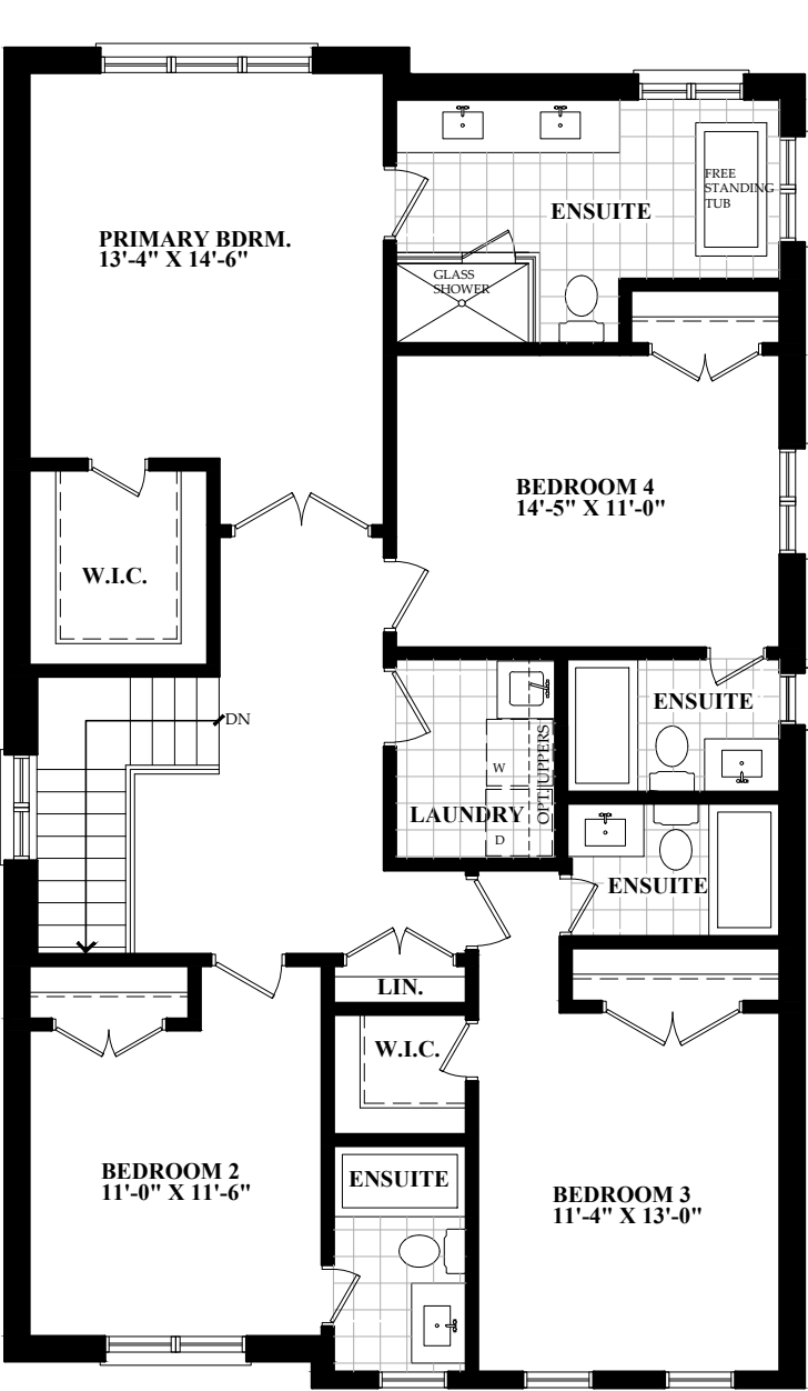
SECOND FLOOR
