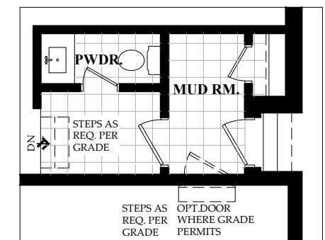
ALT. POWDER LOCATION
