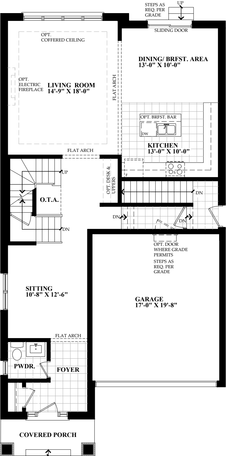
FIRST FLOOR
