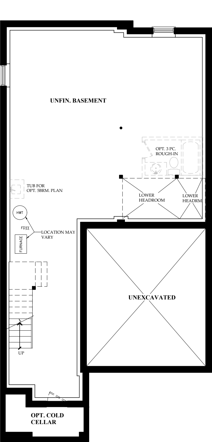
BASEMENT
