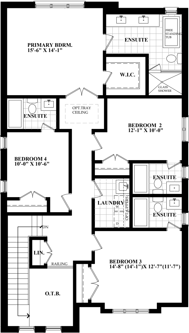
SECOND FLOOR
