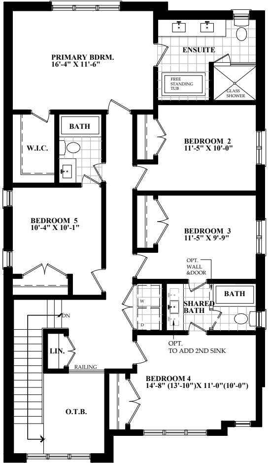
SECOND FLOOR /OPT. 5 BDRM.
