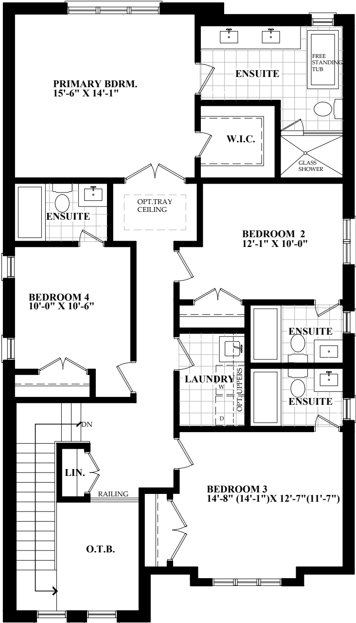
SECOND FLOOR
