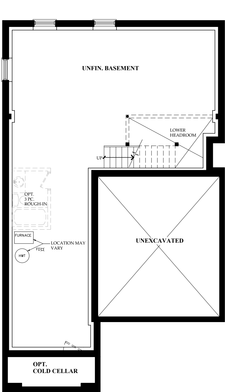
BASEMENT
