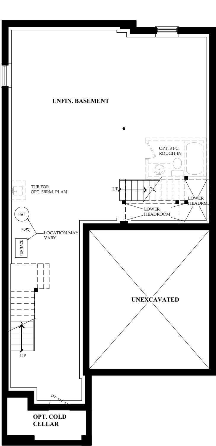
BASEMENT
