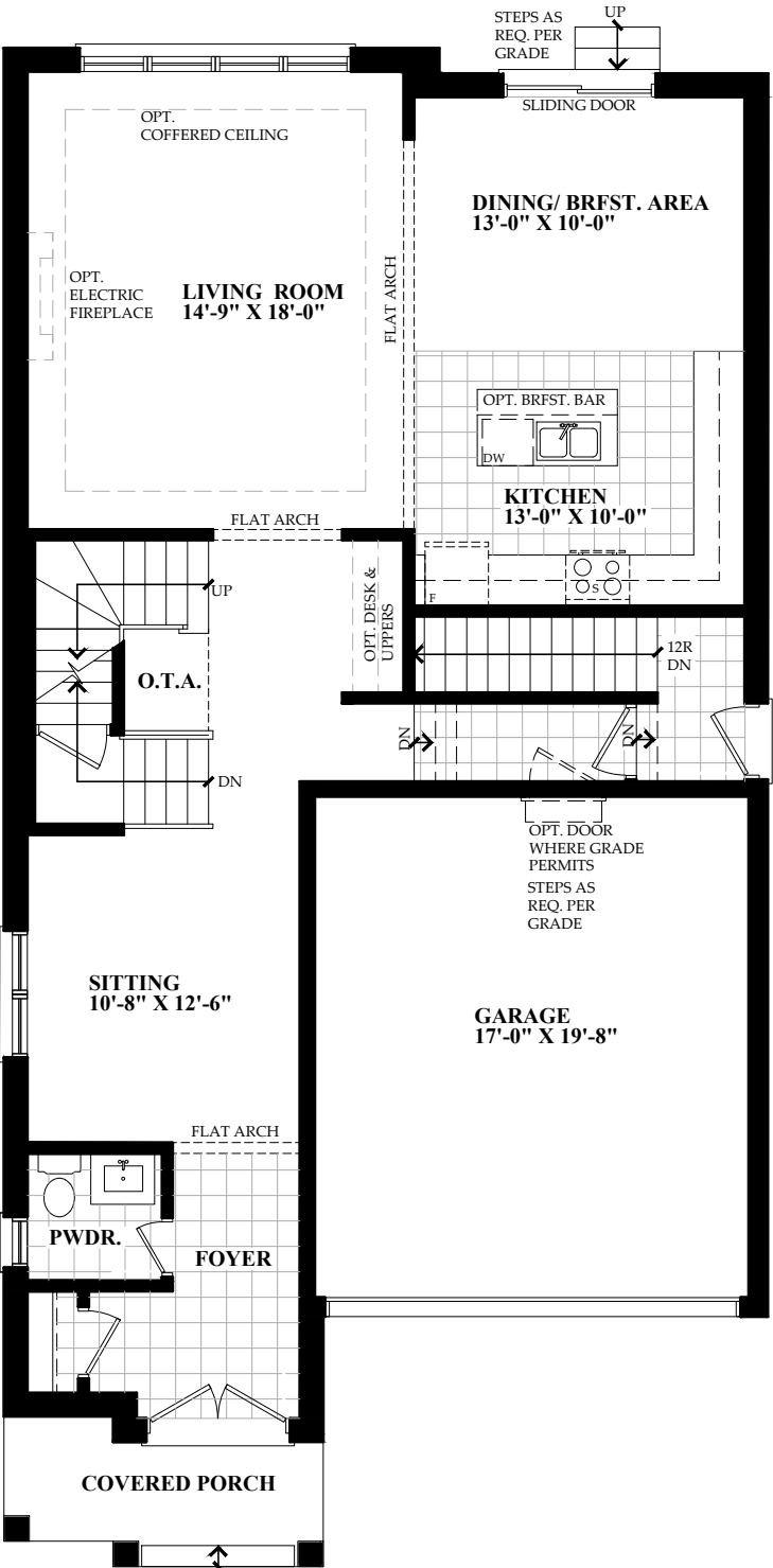
FIRST FLOOR
