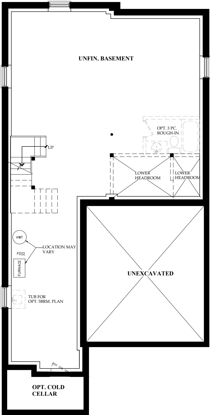
BASEMENT
