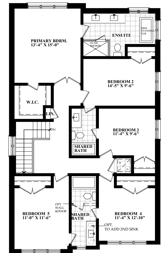
SECOND FLOOR /OPT. 5 BDRM.
