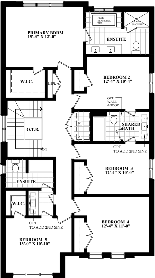
SECOND FLOOR/OPT. 5 BDRM.
