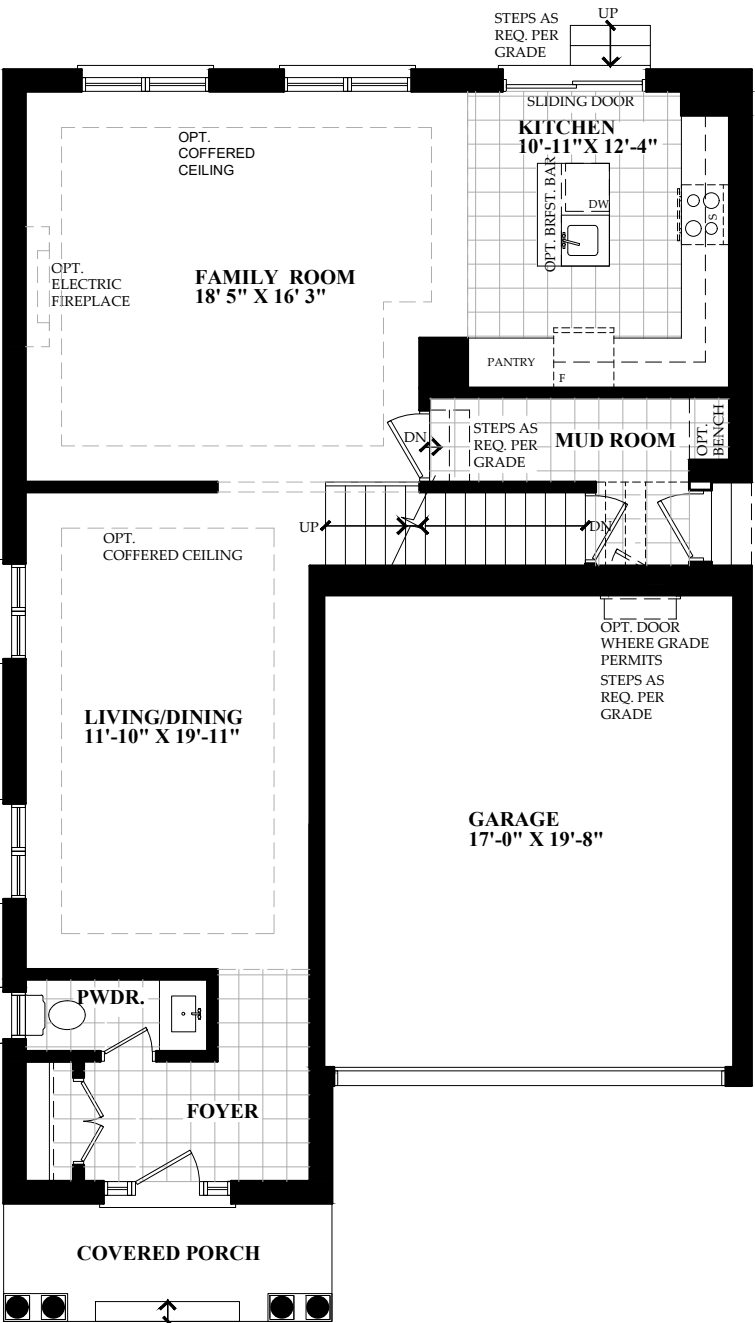
FIRST FLOOR
